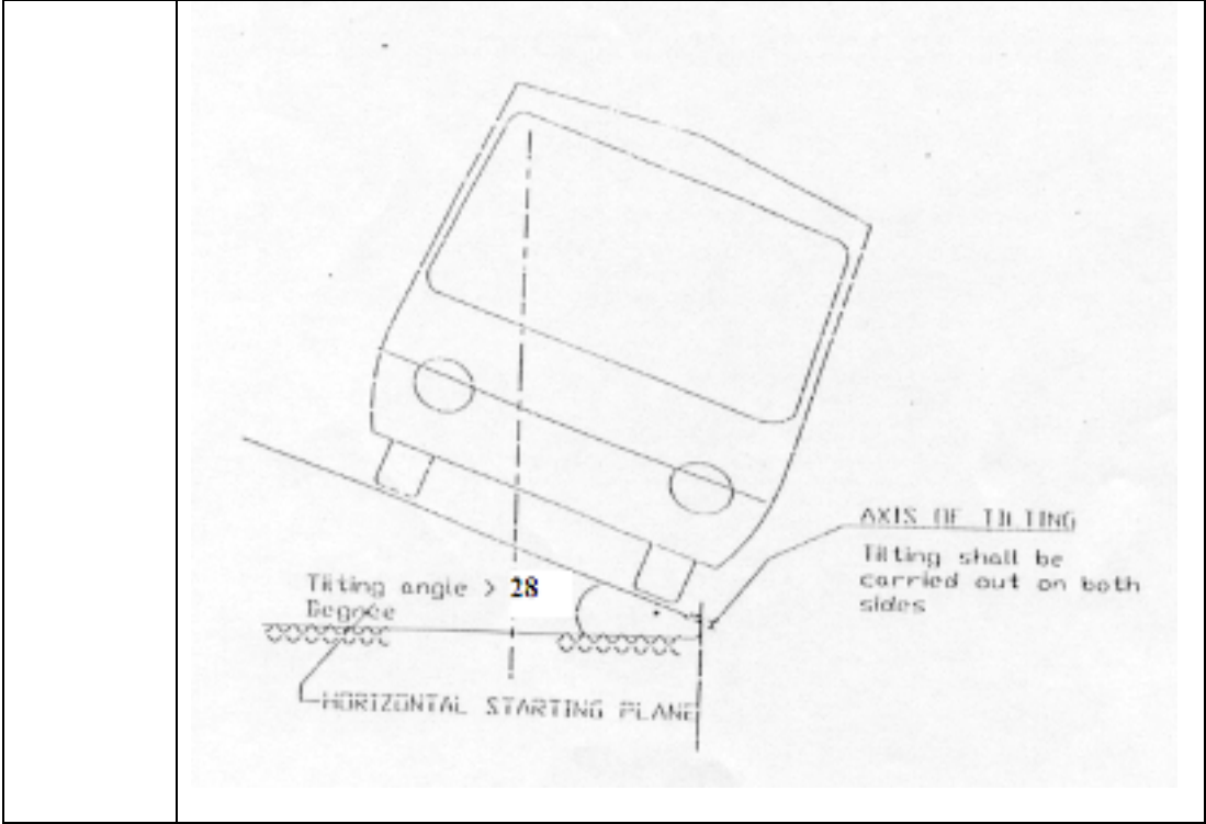
Figure 8 Stability Test and Tilt angle
